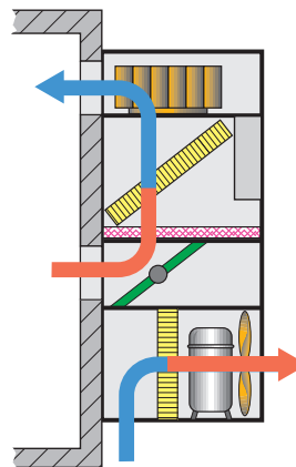
Cooling with compressor
